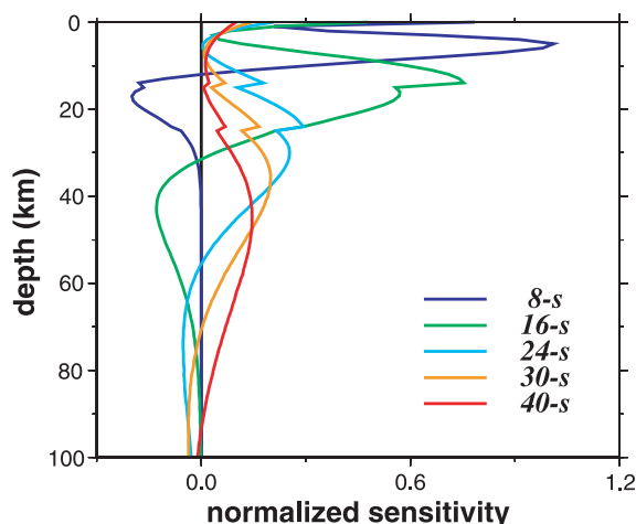
Figure 6. Depth sensitivity of 8-, 16-, 24-, 30-, and 40-s Rayleigh group wave periods.
